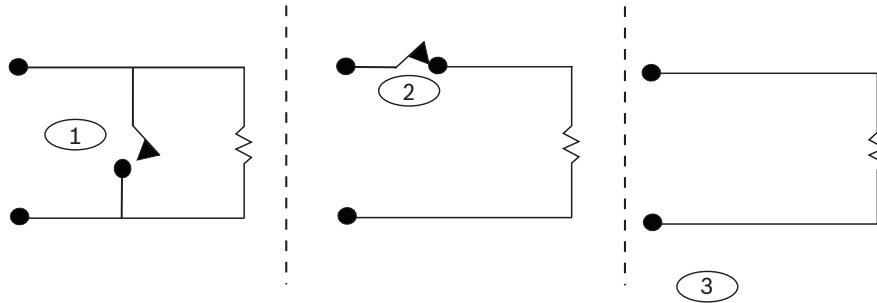
Figure 13.1: Single EOL resistor option
